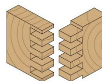
Box joint
